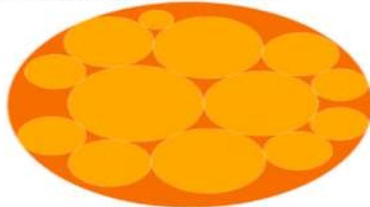
Top 10 WebFrameWorkedWith
