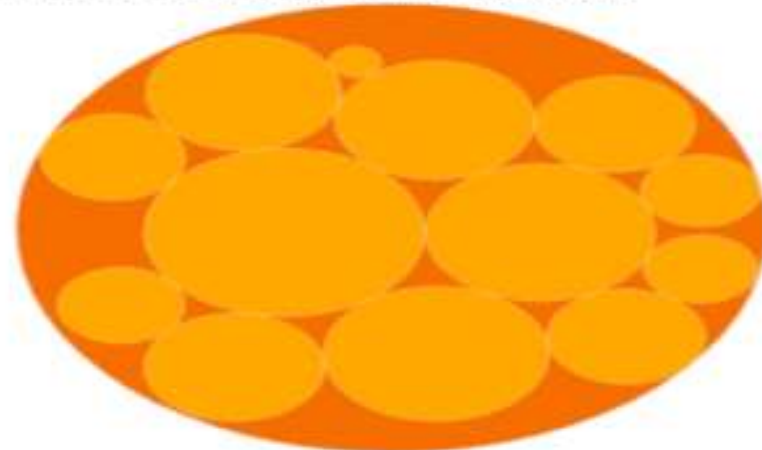
Top 10 WebFrameDesireNextYear
